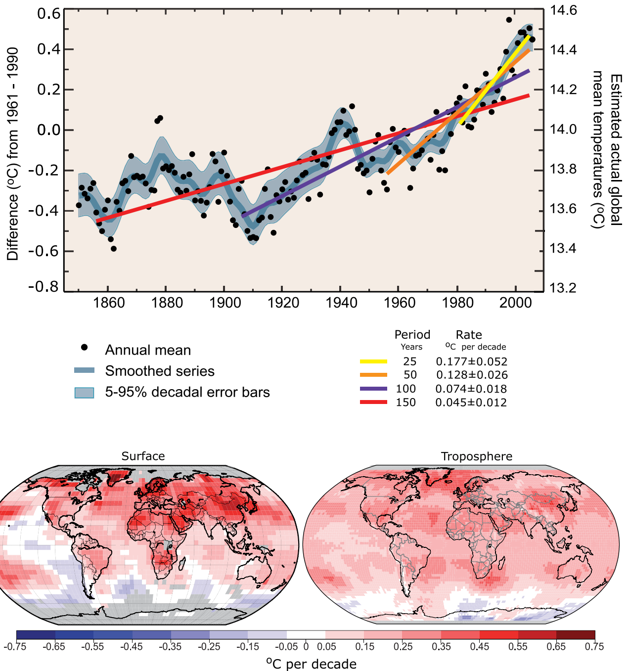
FAQ 3.1, Figure 1. (Top) Annual global mean observed temperatures 1 (black dots) along with simple fits to the data. The left hand axis shows anomalies relative to the 1961 to 1990 average and the right hand axis shows the estimated actual temperature (°C). Linear trend fits to the last 25 (yellow), 50 (orange), 100 (purple) and 150 years (red) are shown, and correspond to 1981 to 2005, 1956 to 2005, 1906 to 2005, and 1856 to 2005, respectively. Note that for shorter recent periods, the slope is greater, indicating accelerated warming. The blue curve is a smoothed depiction to capture the decadal variations. To give an idea of whether the fluctuations are meaningful, decadal 5% to 95% (light grey) error ranges about that line are given (accordingly, annual values do exceed those limits). Results from climate models driven by estimated radiative forcings for the 20th century (Chapter 9) suggest that there was little change prior to about 1915, and that a substantial fraction of the early 20th-century change was contributed by naturally occurring influences including solar radiation changes, volcanism and natural variability. From about 1940 to 1970 the increasing industrialisation following World War II increased pollution in the Northern Hemisphere, contributing to cooling, and increases in carbon dioxide and other greenhouse gases dominate the observed warming after the mid-1970s. (Bottom) Patterns of linear global temperature trends from 1979 to 2005 estimated at the surface (left), and for the troposphere (right) from the surface to about 10 km altitude, from satellite records. Grey areas indicate incomplete data. Note the more spatially uniform warming in the satellite tropospheric record while the surface temperature changes more clearly relate to land and ocean.
