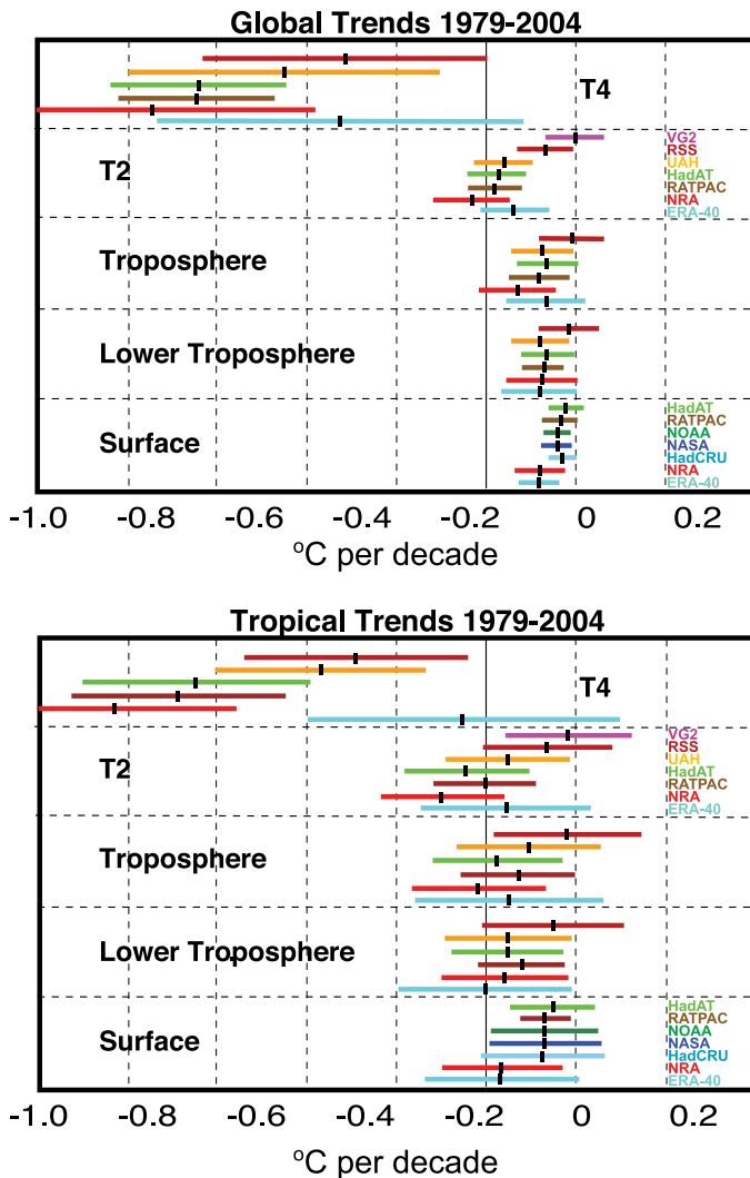
Figure 3.18. Linear temperature trends ( ^{\circ}\text{C} per decade) for 1979 to 2004 for the globe (top) and tropics ( 20^{\circ}\text{N} to 20^{\circ}\text{S} ; bottom) for the MSU channels T4 (top panel) and T2 (second panel) or equivalent for radiosondes and reanalyses; for the troposphere (third panel) based on T2 with T4 used to statistically remove stratospheric influences (Fu et al., 2004a); for the lower troposphere (fourth panel) based on the UAH retrieval profile; and for the surface (bottom panel). Surface records are from NOAA/NCDC (green), NASA/GISS (blue) and HadCRUT2v (light blue). Satellite records are from UAH (orange), RSS (dark red) and VG2 (magenta); radiosonde-based records are from NOAA RATPAC (brown) and HadAT2 (light green); and atmospheric reanalyses are from NRA (red) and ERA-40 (cyan). The error bars are 5 to 95% confidence limits associated with sampling a finite record with an allowance for autocorrelation. Where the confidence limits exceed -1 , the values are truncated. ERA-40 trends are only for 1979 to August 2002. Data from Karl et al. (2006; D. Seidel courtesy of J. Lanzante; and J. Christy).
