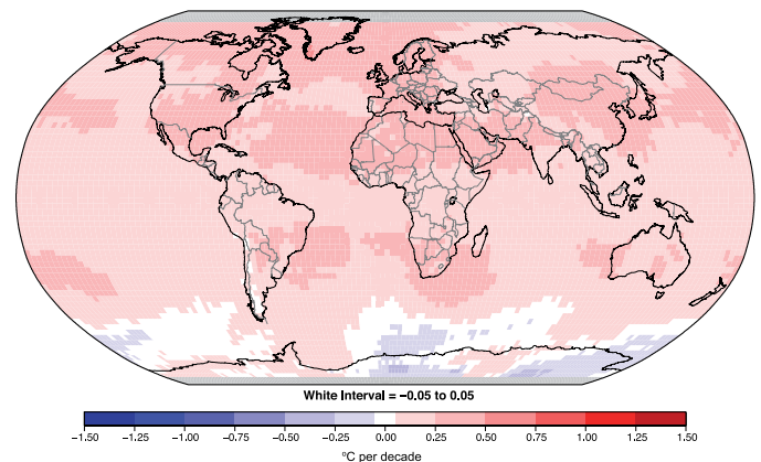
Figure 3.19. Linear tropospheric temperature trends ( ^{\circ}\text{C} per decade) for 1979 to 2005 from RSS (based on T2 and T4 adjusted as in Fu et al., 2004a). Courtesy Q. Fu.
