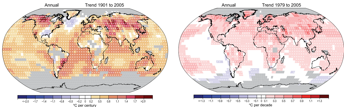
Figure 3.9. Linear trend of annual temperatures for 1901 to 2005 (left; ^{\circ}\text{C} per century) and 1979 to 2005 (right; ^{\circ}\text{C} per decade). Areas in grey have insufficient data to produce reliable trends. The minimum number of years needed to calculate a trend value is 66 years for 1901 to 2005 and 18 years for 1979 to 2005. An annual value is available if there are 10 valid monthly temperature anomaly values. The data set used was produced by NCDC from Smith and Reynolds (2005). Trends significant at the 5% level are indicated by white + marks.
