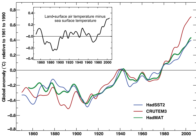
Figure 3.8. Annual anomalies ( ^{\circ}\text{C} ) of global average SST (blue curve, begins 1850), NMAT (green curve, begins 1856) and land-surface air temperature (red curve, begins 1850) to 2005, relative to their 1961 to 1990 means (Brohan et al., 2006; Rayner et al., 2006). The smooth curves show decadal variations (see Appendix 3.A). Inset shows the smoothed differences between the land-surface air temperature and SST anomalies (i.e., red minus blue).
