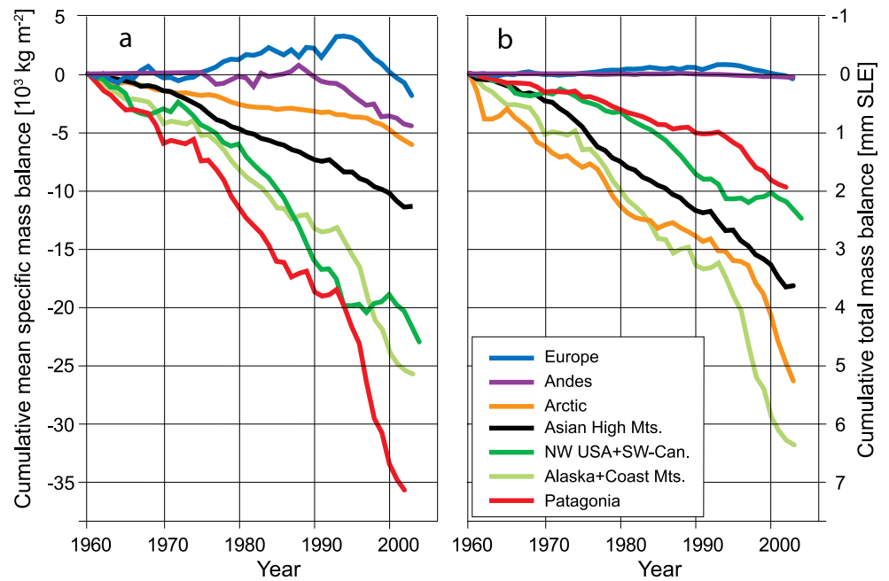
Figure 4.15. Cumulative mean specific mass balances (a) and cumulative total mass balances (b) of glaciers and ice caps, calculated for large regions (Dyrugerov and Meier, 2005). Mean specific mass balance shows the strength of climate change in the respective region. Total mass balance is the contribution from each region to sea level rise.
